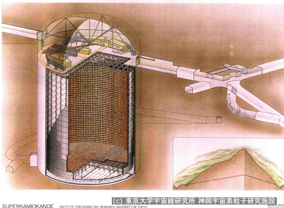
Figure 2 A cutaway drawing of the Super-Kamiokande Detector. The detector is a 40m diameter by 40m high cylinder filled with ultrapure water and surrounded by more than 10,000 50cm phototubes (PMTs), each sensitive enough to see a single photon.
