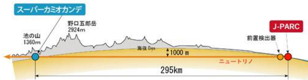
Figure 1 A schematic of a neutrino's journey from the neutrino beamline at J-PARC, through the near detectors (yellow dot) which are used to determine the properties of the neutrino beam, and then 295 km underneath Japan to Super-Kamiokande.
