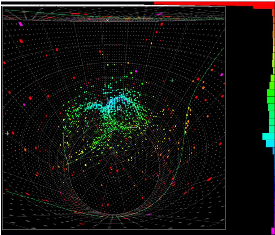
Figure 3 The first T2K event seen in Super-Kamiokande. Each dot is a PMT which has detected light. The two circles of hits indicate that a neutrino has probably produced a particle called a \pi^0 , perfectly in time with the arrival of a pulse of neutrinos from J-PARC. Another faint circle surrounds the viewpoint of this image, showing a third particle was created by the neutrino.
